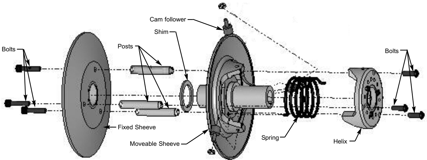
Figure 1--Reverse Driven
